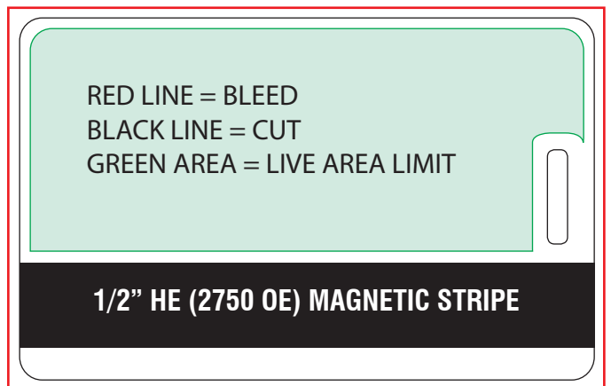
CR80 BACK WITH MAG AND SLOT
